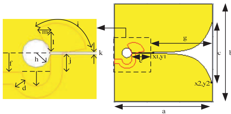
Figure 1: (a) Coplanar Vivaldi, (b) AVA, (c) BAVA.
