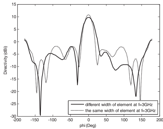
Figure 7: Comparison directivity at f = 3 GHz.
