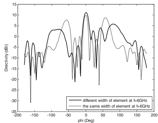
Figure 10: Comparison directivity at f = 6 GHz.
