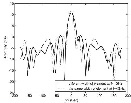
Figure 8: Comparison directivity at f = 4 GHz.
