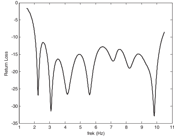
Figure 5: Return Loss UWB antenna (2–10 GHz).
